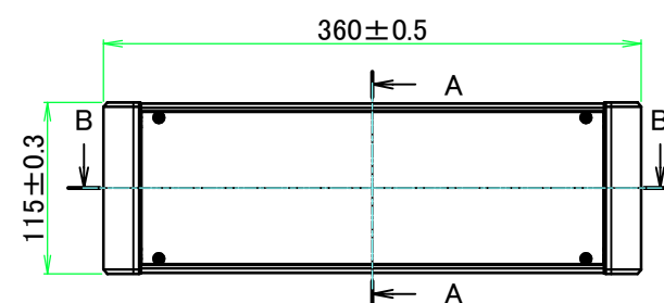
A view
