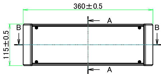
A view
