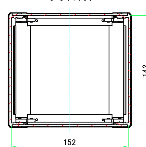
C-C (1:3)
