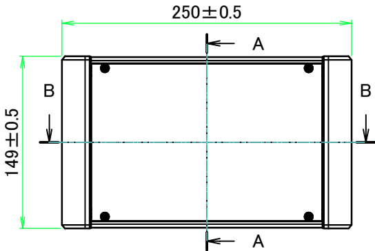
A view
