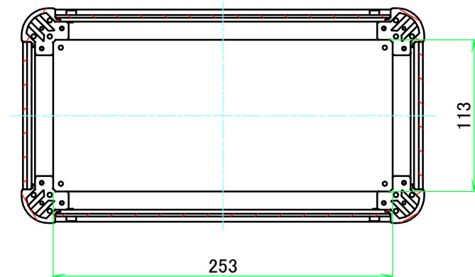
B-B (1:4)
