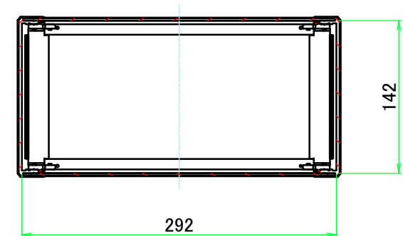
C-C (1:5)
