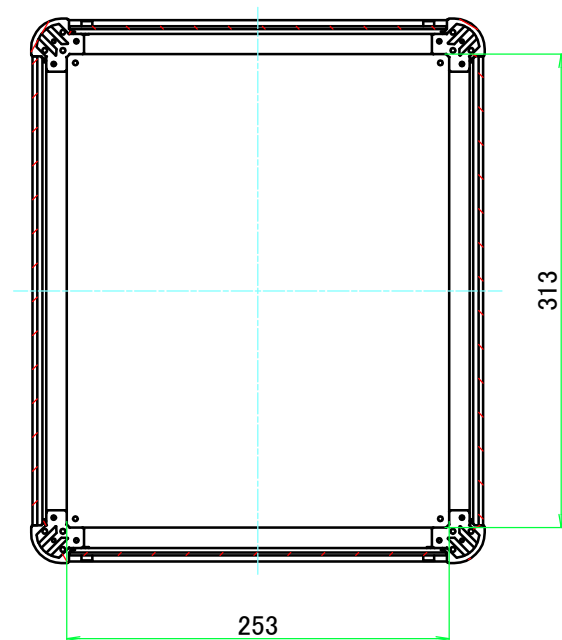
B-B (1:5)
