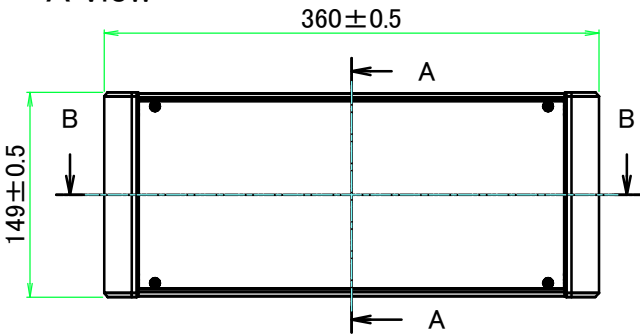
A view
