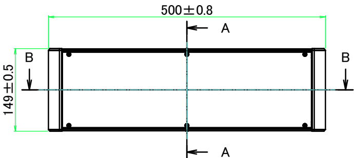
A view
