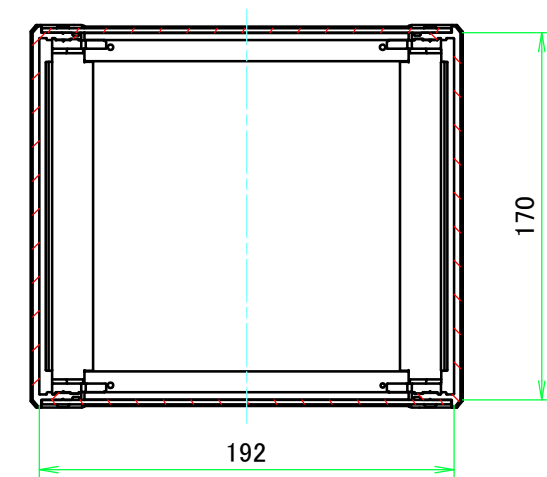
C-C ( 1 :3.5 )
