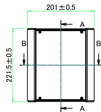
A view
