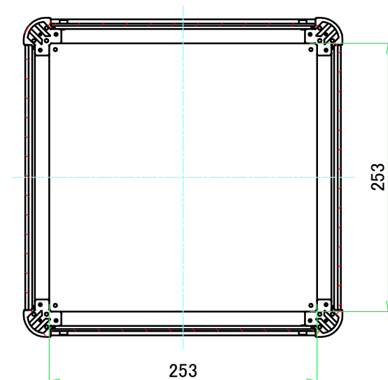
B-B (1:5)
