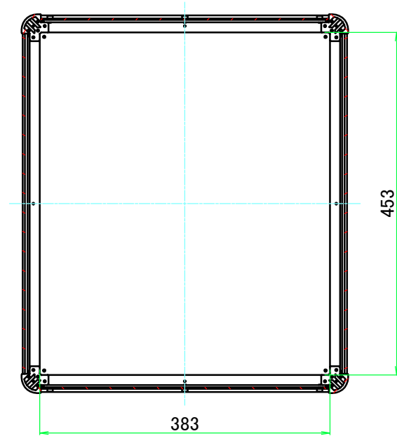
B-B (1:7)
