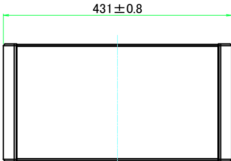
C view
