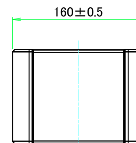
C view
