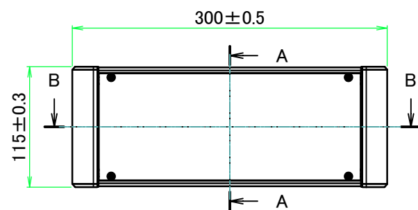
A view
