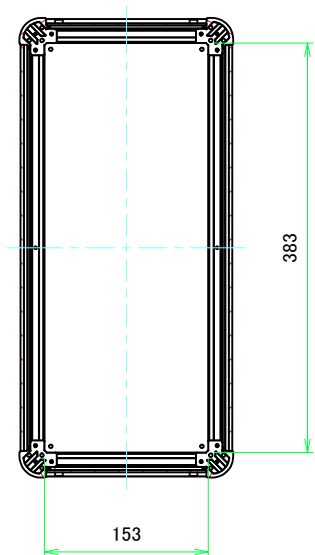
B-B (1:5)
