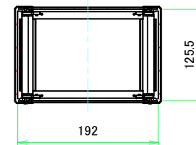
C-C (1:5)
