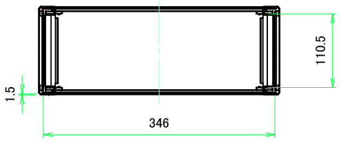
A-A (1:5.5)
