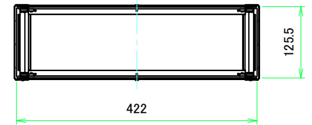
C-C (1:6.5)
