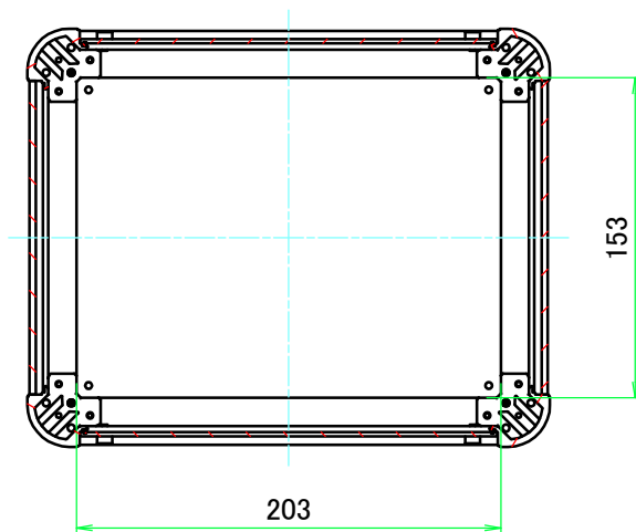
B-B (1:4)
