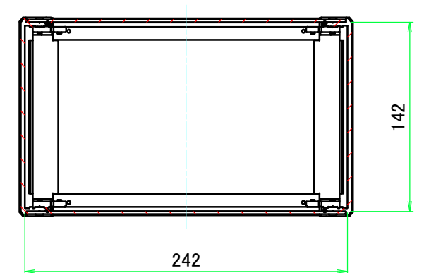
C-C (1:4)
