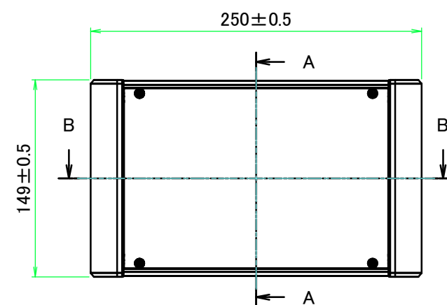
A view
