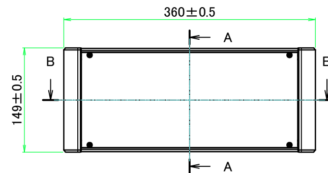
A view
