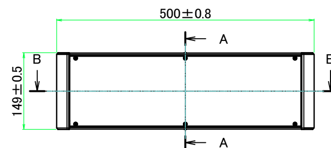
A view
