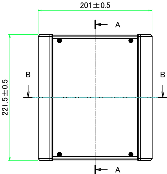
A view
