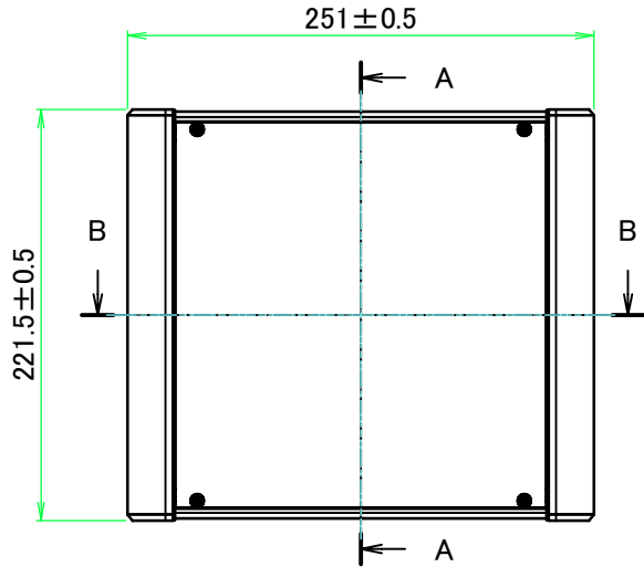
A view
