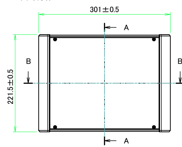
A view
