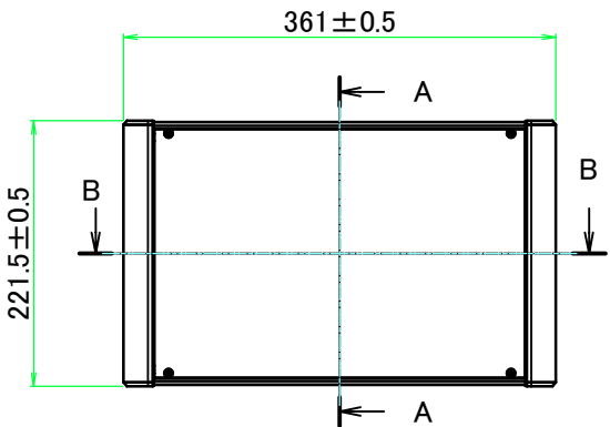
A view
