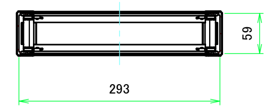
C-C ( 1:5.5 )
