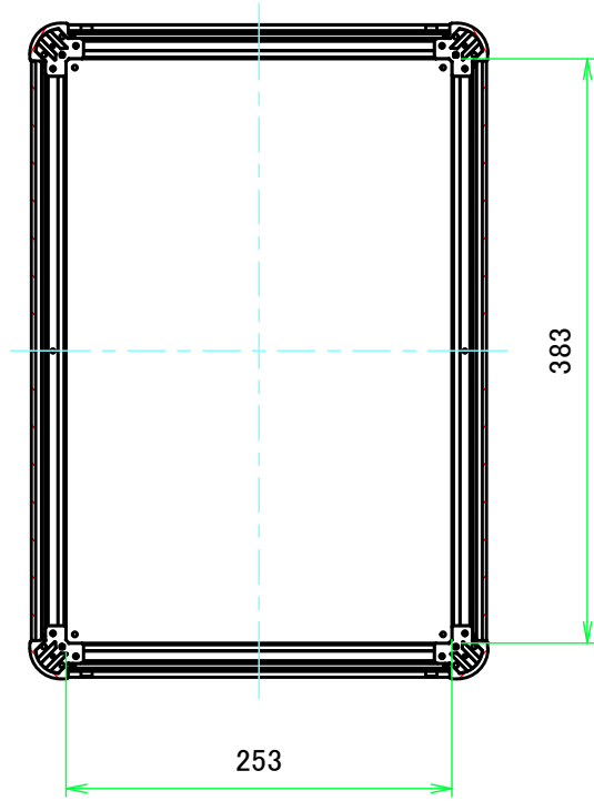
D view
