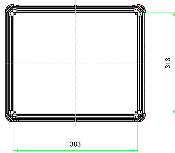
B-B (1:6)
