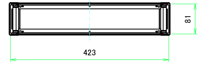
C-C (1:6)
