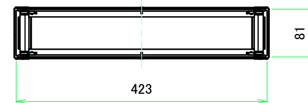
C-C (1:6.5)
