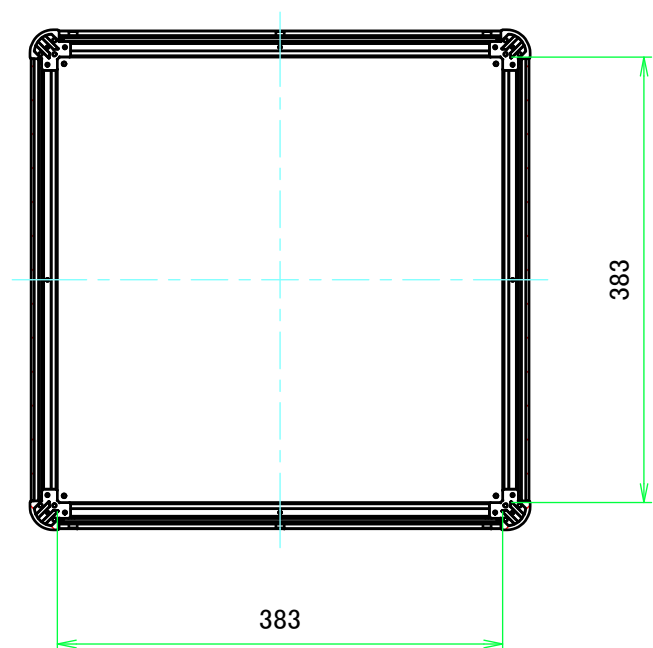
B-B (1:6.5)
