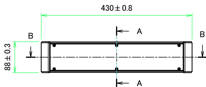
A view
