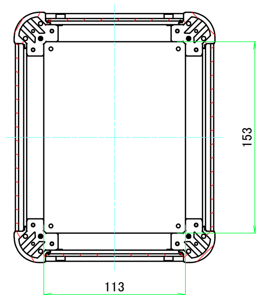
B-B (1:3)
