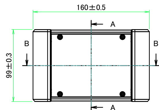
A view
