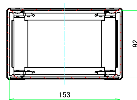
C-C (1:3)
