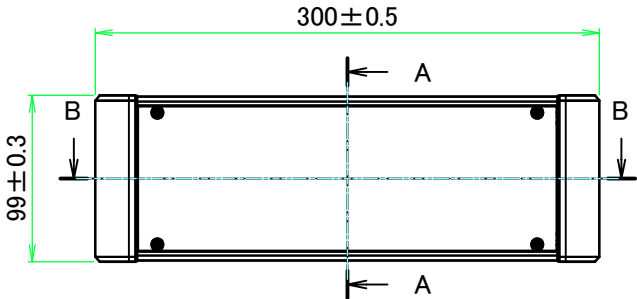
A view
