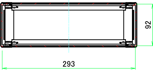
C-C (1:5)
