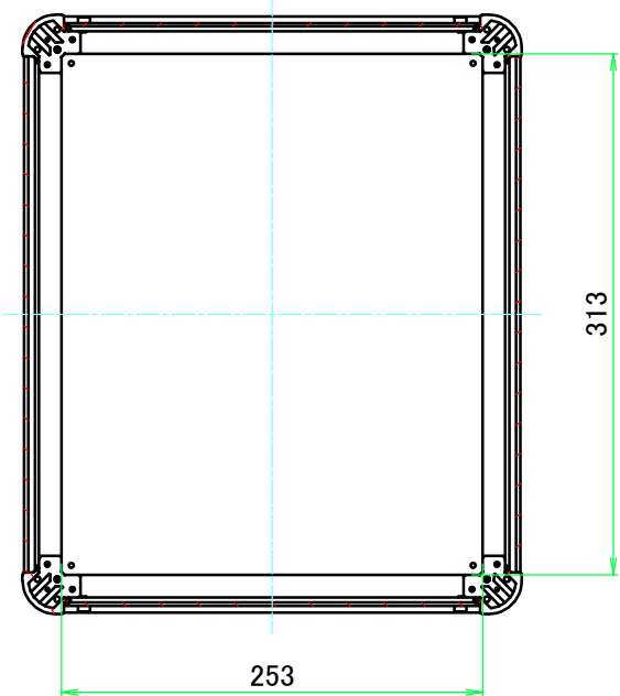
B-B (1:5)
