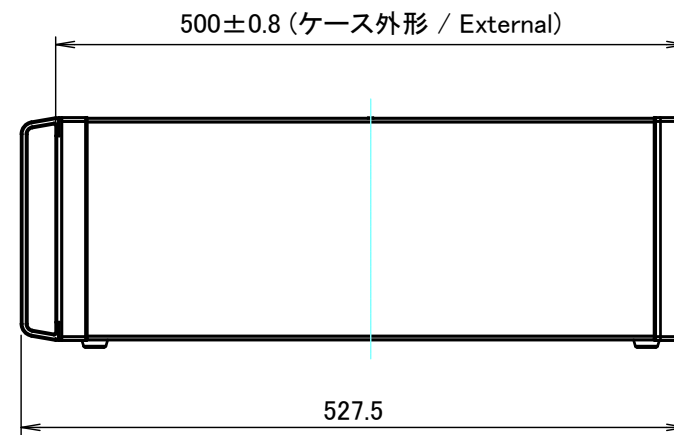
C view
