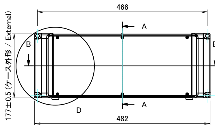
A view
