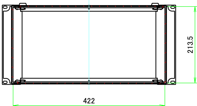
C-C (1:6)
