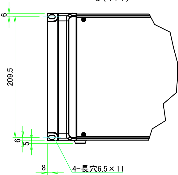
D (1:4)
