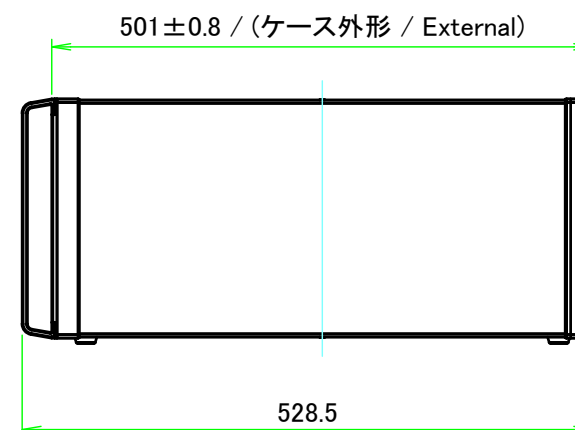
C view
