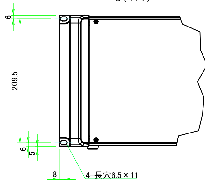
D (1:4)
