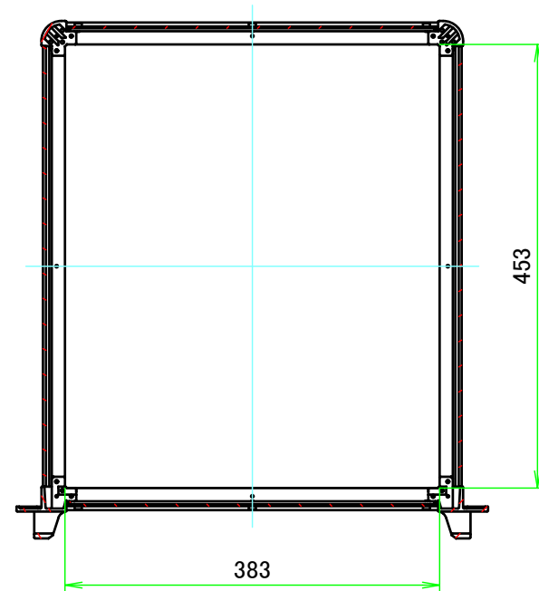
D view
