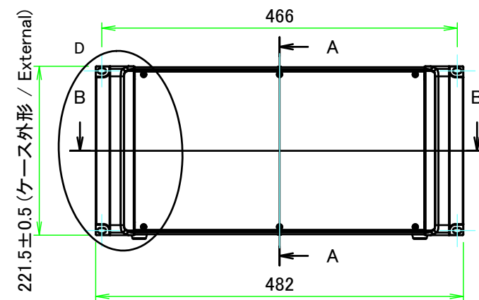
F view
