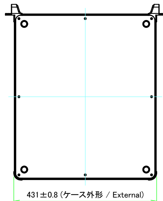
F view
