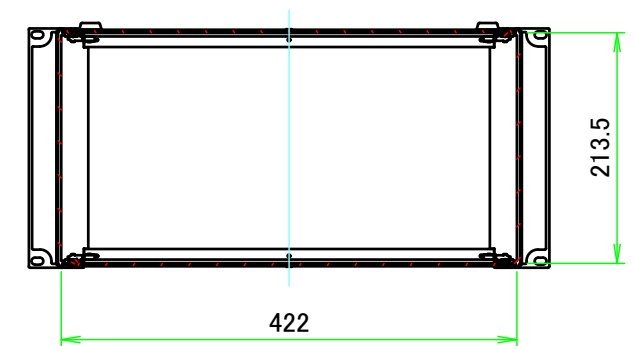
C-C (1:7)
