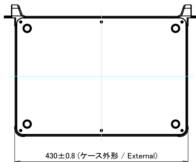
F view
