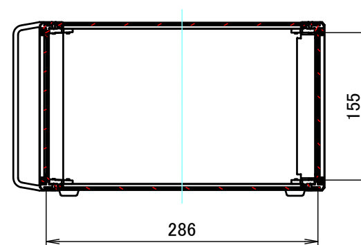
A-A (1:5.5)
