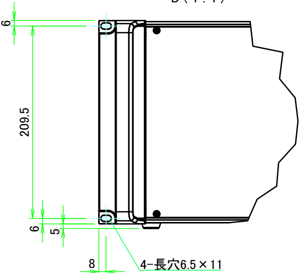
D (1:4)
