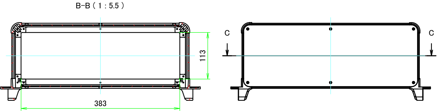
E view
