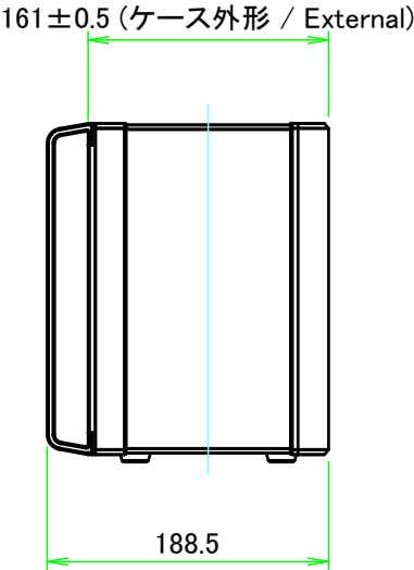
C view
