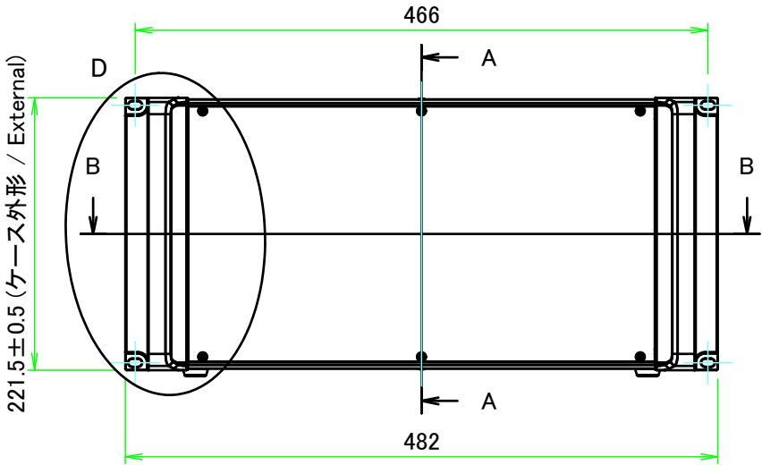
A view
