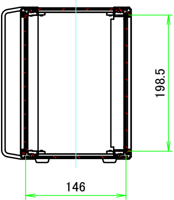
A-A (1:5.5)
