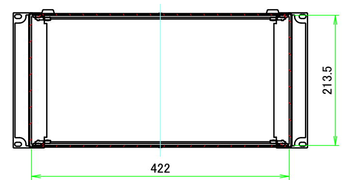
C-C (1:6)
