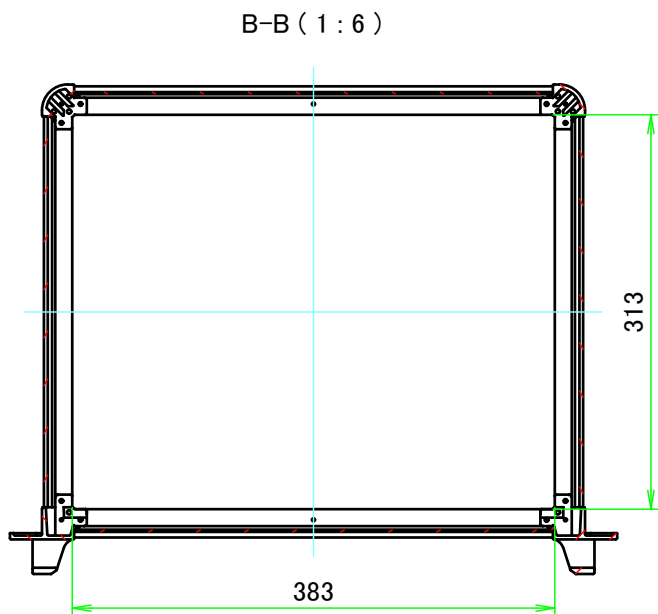
D view
