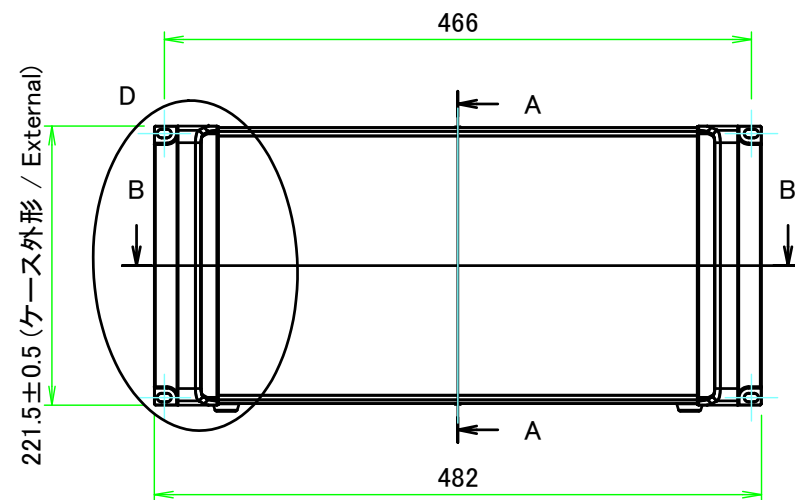
A view
