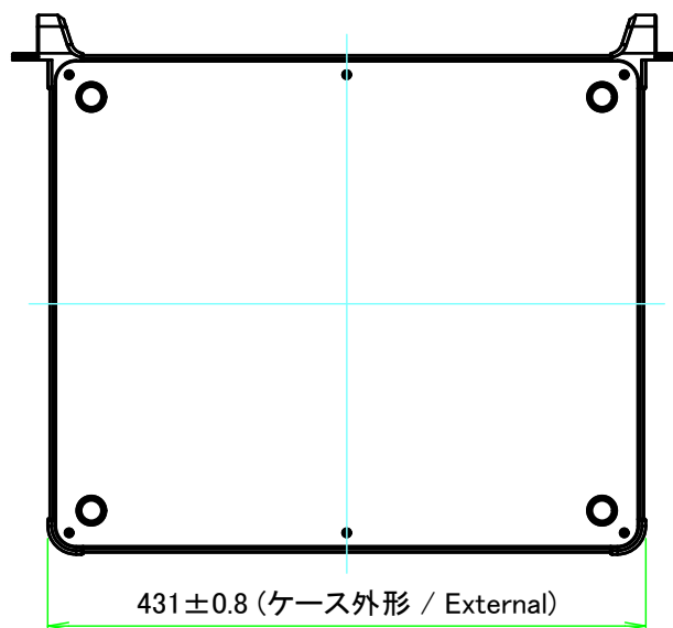
F view
