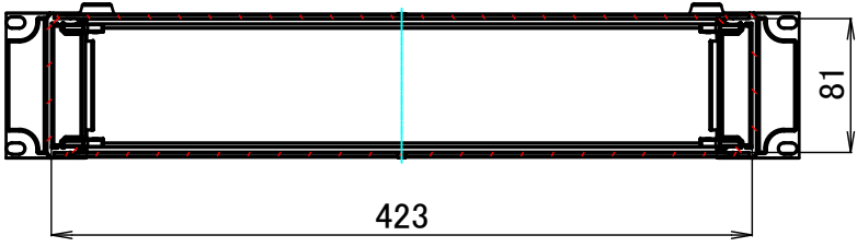
C-C (1:5)
