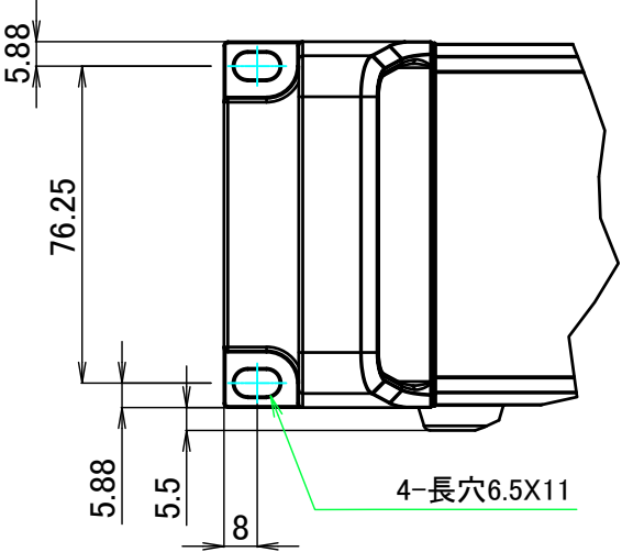
D (1:2)
