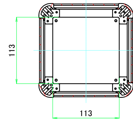
C-C (1:4)
