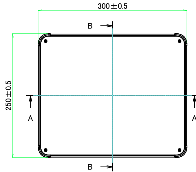
A view
