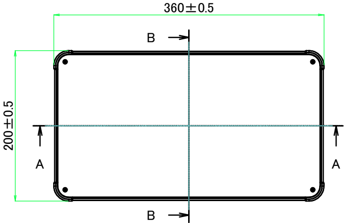
E view
