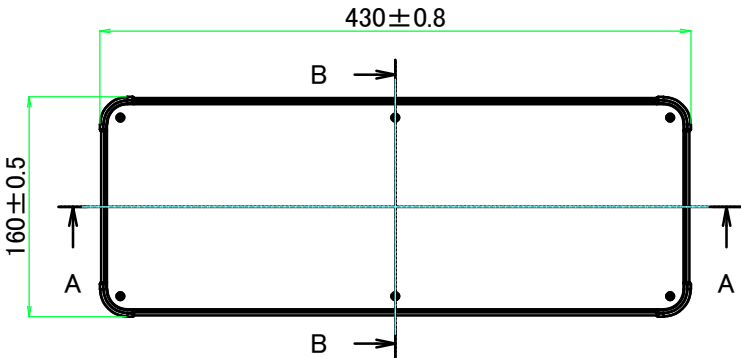
E view
