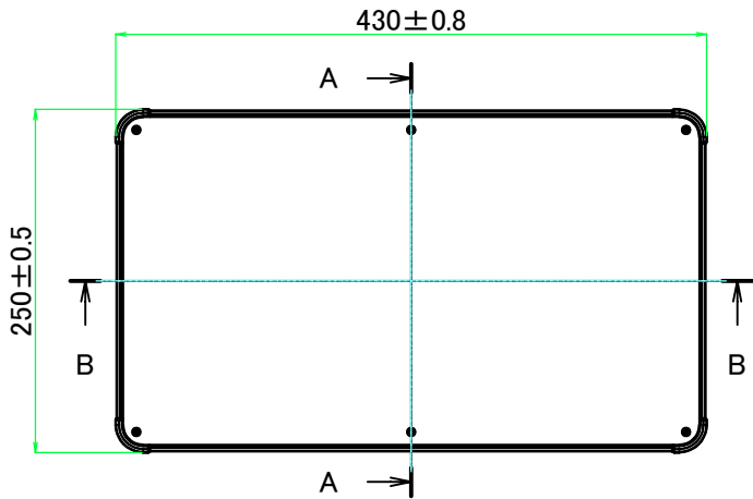
E view
