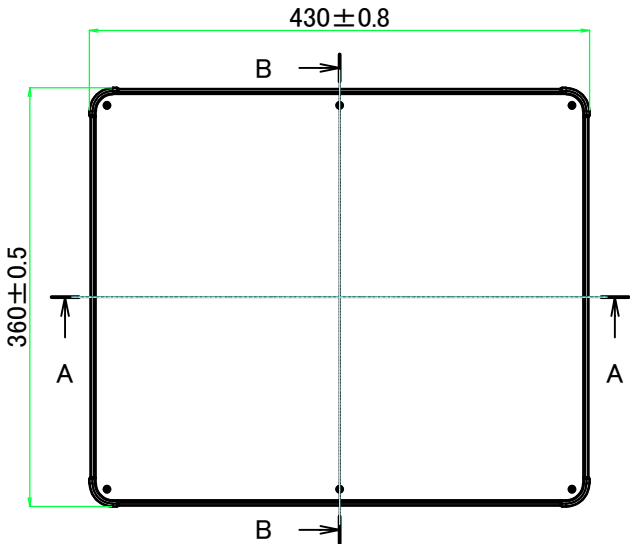
E view
