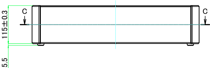
A view
