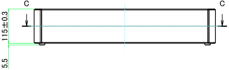
A view
