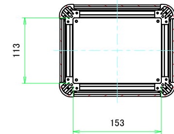
C-C (1:4.5)
