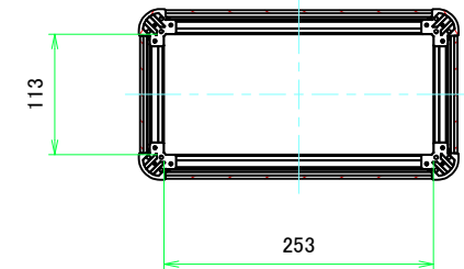
C-C (1:5.5)
