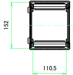
A-A (1:5.5)
