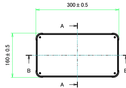
E view
