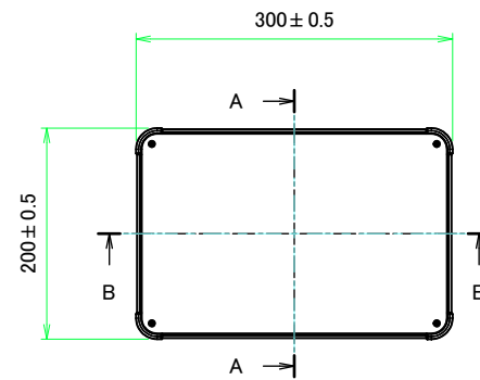
E view
