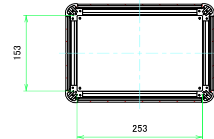
C-C (1:5.5)
