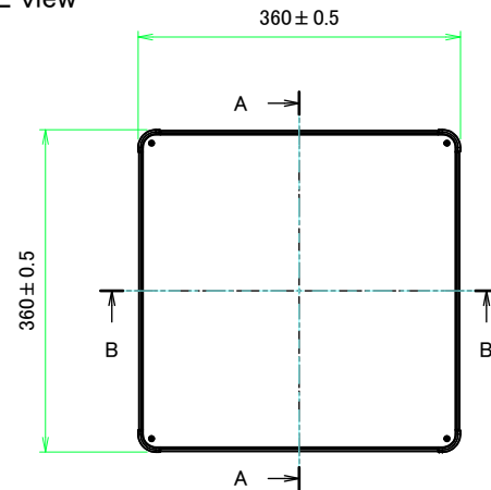
E view
